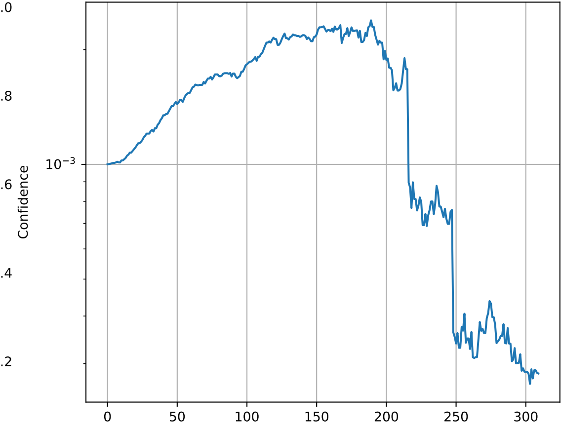
Action Probability Evolution
